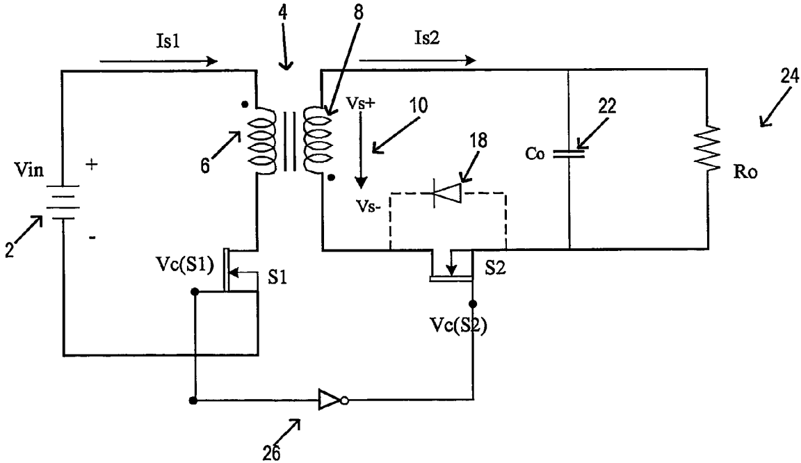
Fig. 1 Prior Art
