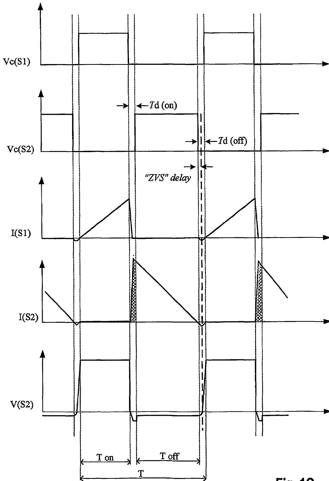
Fig. 1C Prior Art
